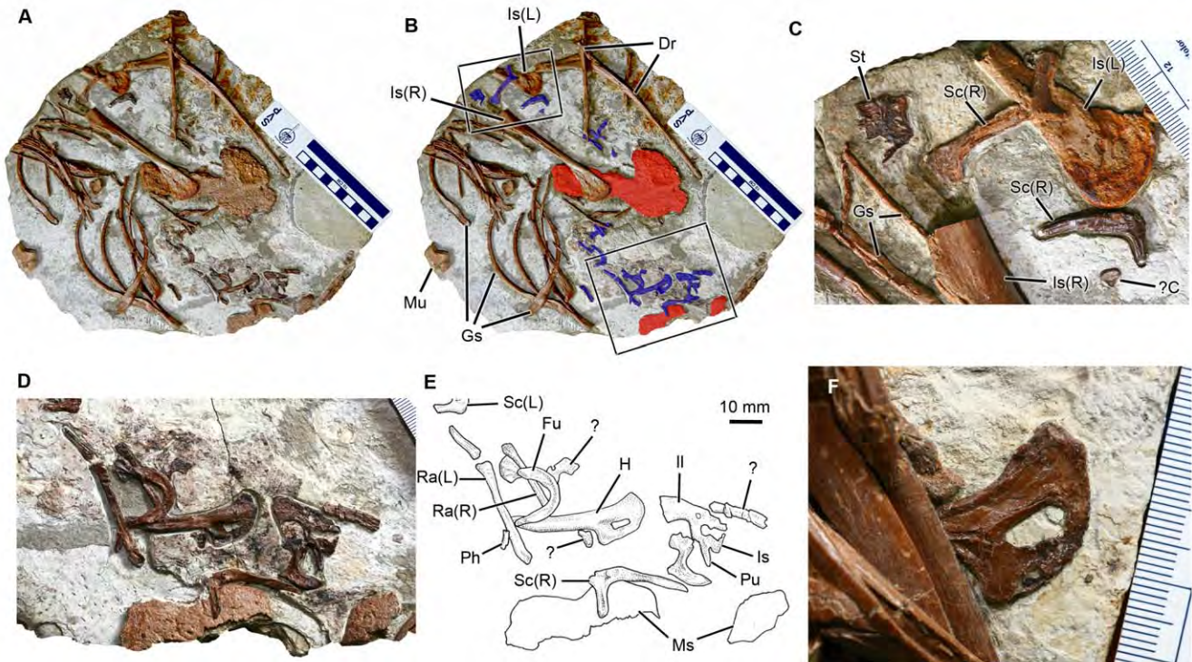
Figure 3. Abdominal contents of Sinocallopteryx gigas (CAGS-IG-T1). A, B; block containing Confuciusornis (blue) and unidentified ornithischian (red) remains. C, Close up of Confuciusornis sternal and pectoral elements (small box in B); D, E; associated skeleton of Confuciusornis (large box in B); F, proximal Confuciusornis humerus (arrow in Figure 2). Abbreviations: C, carpal; Dr, dorsal rib; Fu, furcula; Gs, gastralgia; H, humerus; Il, ilium; Is, ischium; Mu, manual ungula; Ms, miscellaneous ornithischian bone; Ph, phalanx; Pu, pubis; Ra, radius; Sc, scapulocoracoid; St, sternum. Scale bars in A, B equal 10 cm in 1 cm increments; C, F in 1 mm increments. doi:10.1371/journal.pone.0044012.g003
