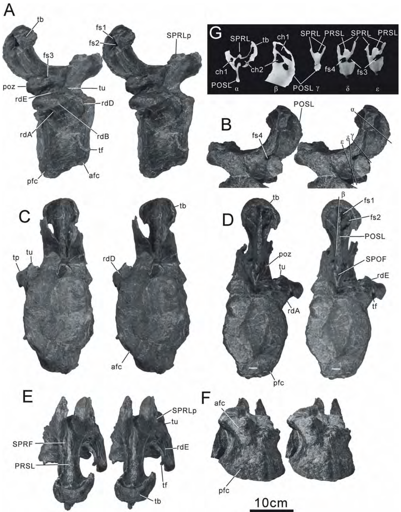
FIGURE 12. Tambatitanis amicitiae gen. et sp. nov., holotype (MNHAH D-1029280). A–F, stereopairs of Cd4. A, right lateral view. B, left lateral view of the neural spine. C, anterior view. D, posterior view. E, dorsal view. F, ventral view. G, CT slices through the neural spine of Cd4, part corresponding to the matrix that filling the internal chamber is removed from the image. Greek letters in B and D indicate the position of CT slices shown in G. Scale bar = 10cm. See text for abbreviations.
