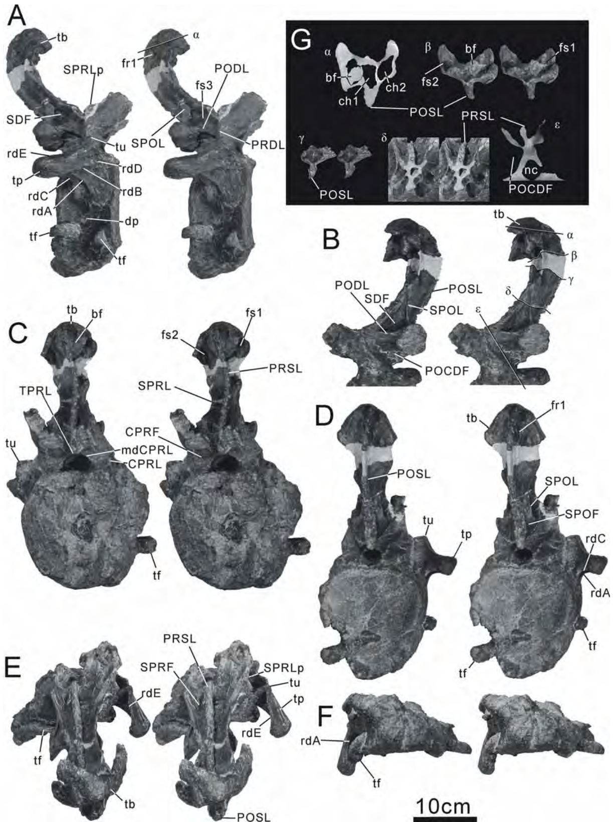
FIGURE 10. Tambatitanis amicitiae gen. et sp. nov., holotype (MNHAH D-1029280). A–F , stereopairs of Cd2. A , right lateral view. B , left lateral view of the neural spine. C , anterior view. D , posterior view. E , dorsal view. F , ventral view. G , CT slices and stereopairs of the breakage section of the neural spine of Cd2, part corresponding to the matrix that filling the internal chamber is removed from the CT image. Greek letters in A and B indicate the position of CT slices and the stereopairs of the breakage surface of the spine shown in G . Scale bar = 10 cm. See text for abbreviations
