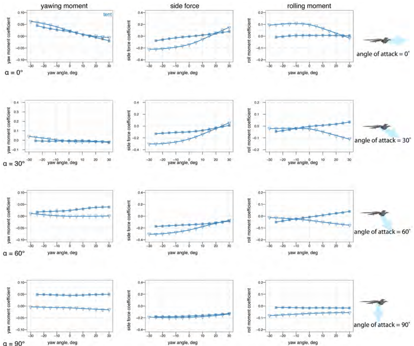
Figure 23. Asymmetric one wing down effect on yaw, tent posture. Baseline tent position (solid square), left wing down (down triangle). Placing one wing down does not make large yawing moments. Some roll and side force is produced at low angles of attack, at the expense of one quarter to one half of the lift. doi:10.1371/journal.pone.0085203.g023
