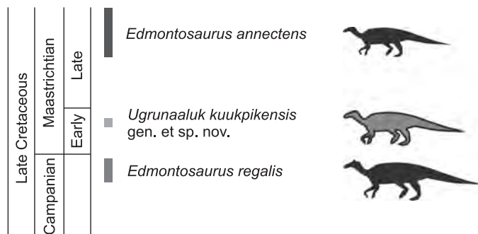
Fig. 2. Temporal distribution of Edmontosaurus species and Ugrunaaluk kuukpikensis gen. et sp. nov. from the Prince Creek Formation in the Late Cretaceous.
