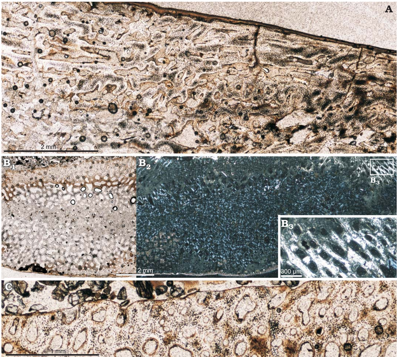
Fig. 5. Bone microstructure of the parietal frill in adult Protoceratops andrewsi Granger and Gregory, 1923, Bayn Dzak, Mongolia, Late Cretaceous (ZPAL MgD-II/33). A . Sagittal section. B , C . Transversal sections; note the condensations of the fossilized collagen fibers strengthening the porous tissue ( B ) and the formation of the small erosion lacunae at the external surface of the frill ( C ). A , B 1 , C , normal light; B 2 , B 3 , polarized light.
