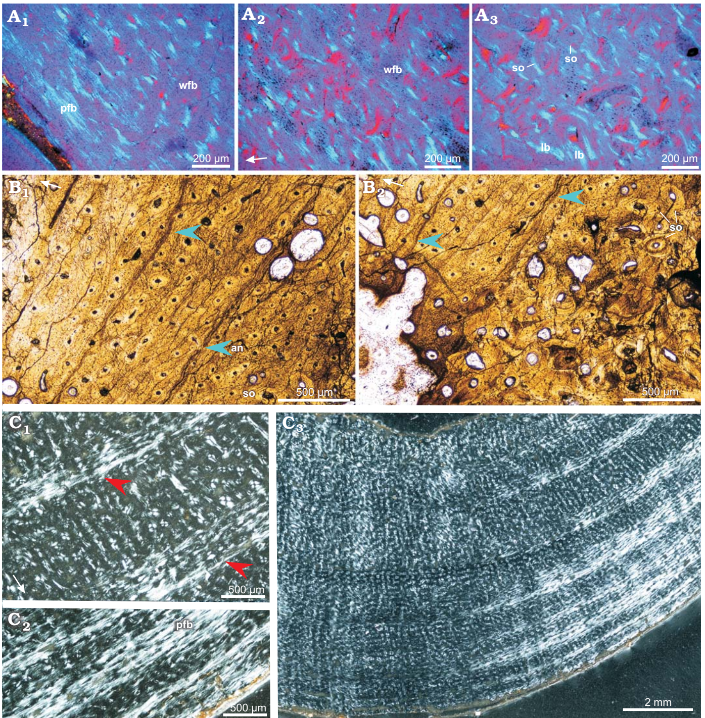
Fig. 9. Bone microstructure in adult Protoceratops andrewsi Granger and Gregory, 1923, Bayn Dzak, Mongolia, Late Cretaceous. A. Ulna ZPAL MgD-II/8, matrix in the outer ( A_1 ) and mid-cortex ( A_2 ), perimedullar region with endosteally-formed lamellar bone ( A_3 ). B. Fibula ZPAL MgD-II/11b; note well formed LAGs (blue arrowheads) and annulus in the cortex ( B_1 ); deeper cortex shows signs of remodeling and multiple secondary osteons ( B_2 ). C. Femur ZPAL MgD-II/11a, compacta showing wider zones of fast growing woven-fibered bone intersected by thin annuli of parallel-fibered bone (red arrowheads) in the mid-cortex ( C_1 , C_3 ); condensation of the parallel-fibered bone zones in the outer cortex ( C_2 ). A. polarized light (quartz wedge); B. normal light; C. polarized light. White arrows point outward. Abbreviations: an, annulus; lb, lamellar bone; pfb, parallel-fibered bone; so, secondary osteons; wfb, woven-fibered.
