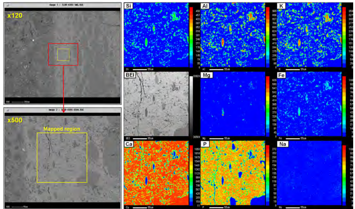
Fig 3. EPMA mapping of the rib bone adjacent to the boundary. Due to calcite and calcium content in the bone region, the distribution and concentration of Ca is very high. The most striking feature is that miniscule pores within the bone matrix and some of the smaller vascular channels are occupied with illite (Al, Si, K, Mg, Fe) instead of calcite. BEI = backscattered electron image.
