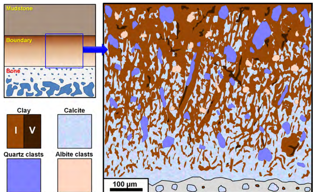
Fig 9. Simplified illustration of the boundary region. The haphazard, reticular orientation of clay and the relatively abundant inclusion of quartz and albite clasts is a notable feature of this region. Clay concentration progressively increases towards the mudstone region, and a thin line of calcite microcrystals covers the bone surface. I = illite, V = vermiculite.
