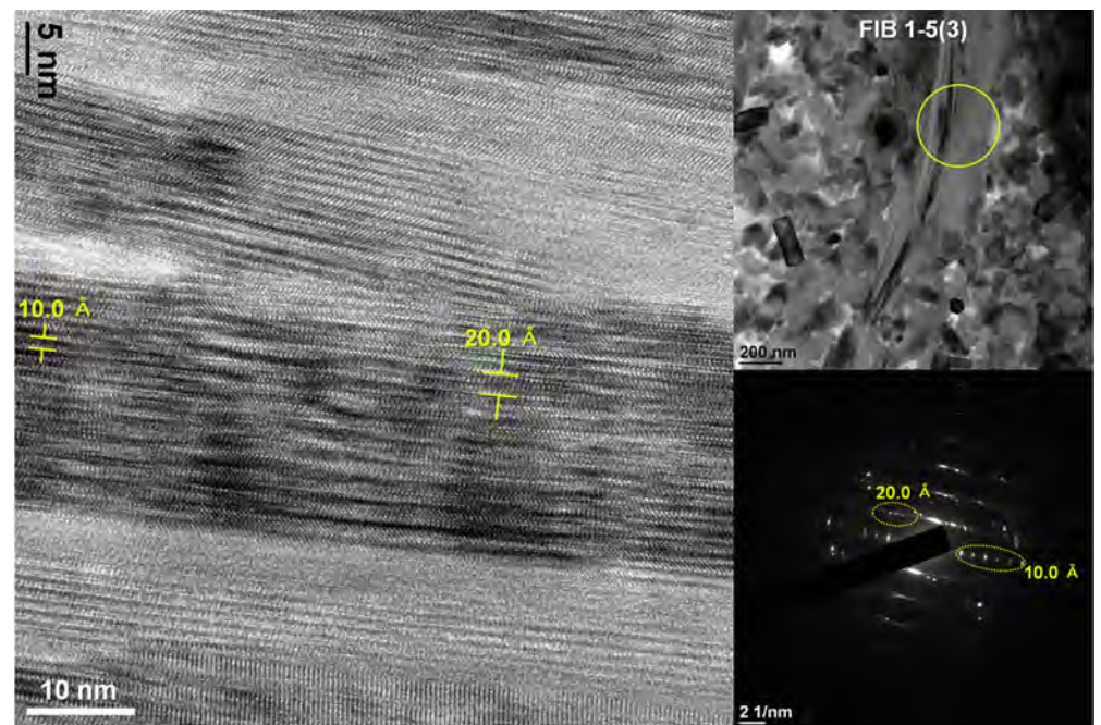
Fig 6. An area showing lateral variation of the 1M-type illite and the 2M-type illite within the same layer. The gradual transformation of the 1M to 2M illite in a lateral direction is apparent. Note the highly disordered {001} lattices of 2M from the HRTEM image.
