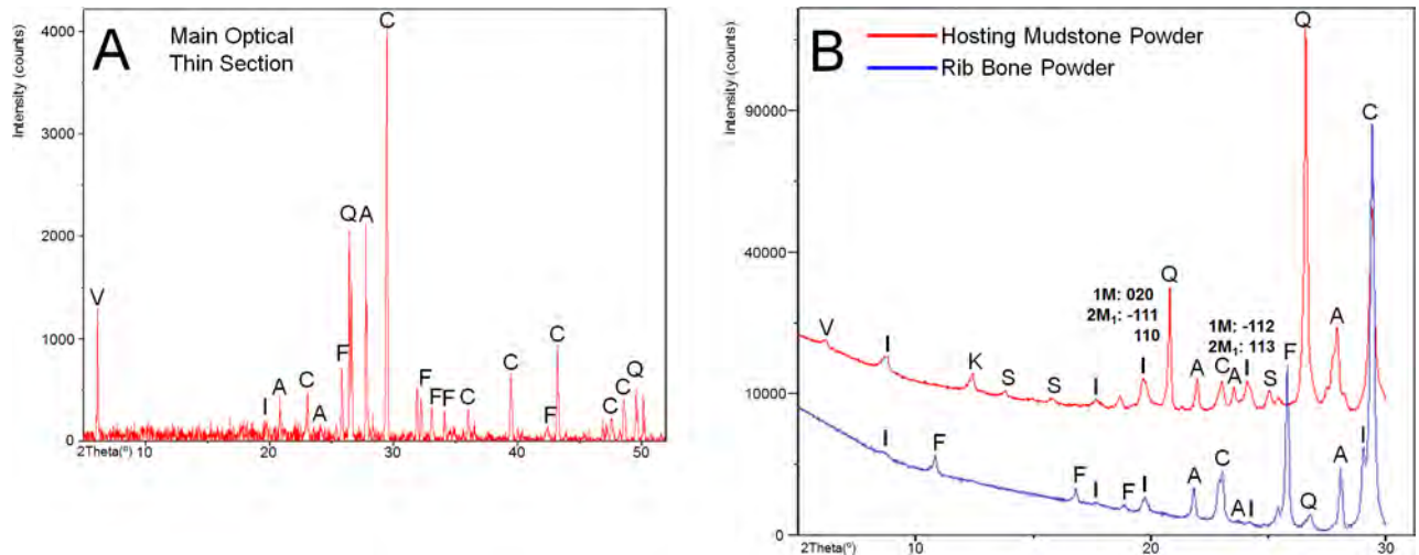
Fig 2. XRD analysis. (A) Main optical thin section (noise background removed). Major phases were calcite, quartz, albite, and fluorapatite. Vermiculite and illite were distinctly identified clay phases. (B) Hosting mudstone powder and rib bone powder focused on identifying clay phases. Clay phases besides illite were not detected from the rib bone sample. The prominent illite peaks at 20° and the peaks in 24° range in the mudstone sample indicate that both 1M and 2M 1 illite polytypes are present. A = albite, C = calcite, F = fluorapatite, I = illite, K = kaolinite, Q = quartz, S = sanidine, V = vermiculite.
