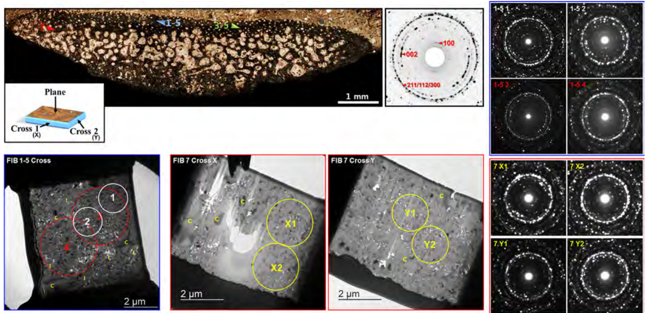
Fig 8. TEM micrographs and SAED patterns of apatite crystals from the selected areas (circles) of FIB 1±5 and FIB 7, obtained from the rib bone matrix. FIB 1±5 was obtained from an area with rich clay content, and all SAED patterns from areas with dense apatite population resulted in moderate to a slightly strong degree of preferred orientation. Both FIB 7 cross samples were milled from areas notably lacking in clay content. Besides cross X1, all SAED patterns lacked preferred orientations. C = calcite, I = illite.
