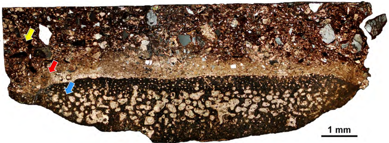
Fig 1. Composite cross-polarized optical micrograph of the main thin section (x40). The section was divided into three regions± hosting mudstone (yellow arrow), boundary (red arrow), and rib bone (blue arrow). Clusters of calcite microcrystals can be directly observed in all regions. The mudstone and boundary region primarily contains detrital clasts of quartz and feldspars. Due to the compressed nature of the bone matrix, specific osteohistological features were not discernible from the rib bone besides the vascularization pattern.
