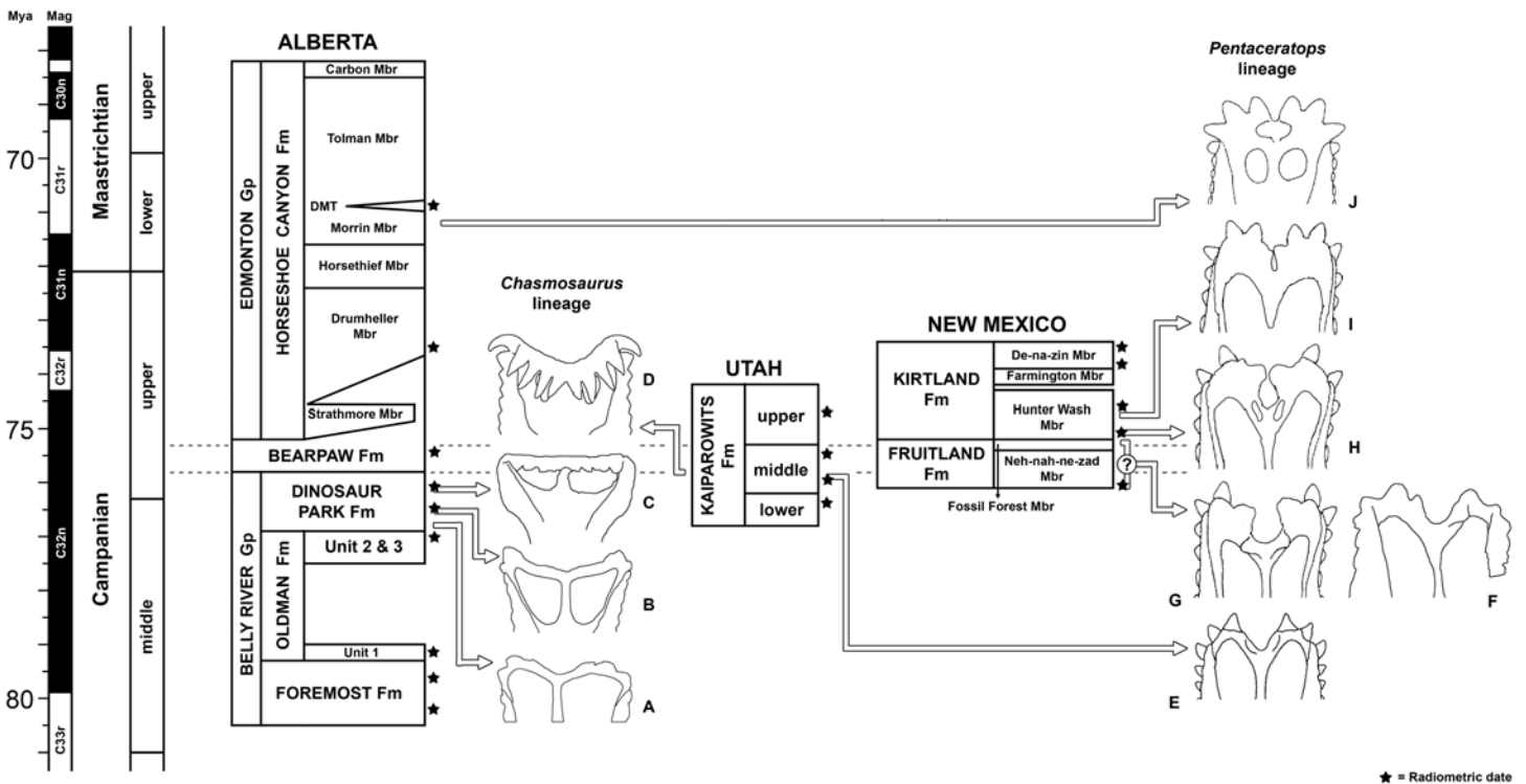
Figure 10 Stratigraphic positions of chasmosaurine taxa. Morphospesies of Chasmosaurus (A–D) and Pentaceratops (E–J) clades which do not overlap stratigraphically. These are hypothesized to form two anagenetic lineages which resulted from a cladogenetic branching event prior to the middle Campanian. (A) “ Chasmosaurus russelli ”, lower Dinosaur Park Fm, ~76.8 Ma. (B) Chasmosaurus belli , middle Dinosaur Park Fm, ~76.5–76.3 Ma. (C) Vagaceratops irvinensis , upper Dinosaur Park Fm, ~76.1 Ma. (D) Kosmoceratops richardsoni , middle Kaiparowits Fm, ~76.0–75.9 Ma. (E) Utahceratops gettyi , middle Kaiparowits Fm, ~76.0–75.6 Ma. (F), c.f. Pentaceratops sternbergii , unknown occurrence within “Fruitland Formation” ~76.0–75.1 Ma. (G) Aff. Pentaceratops n. sp., uppermost Fossil Forest Mbr, Fruitland Fm, ~75.1 Ma. (H) Navajoceratops sullivanii , lowermost Hunter Wash Mbr, Kirtland Fm, ~75.0 Ma. (I) Terminocavus sealeyi , middle Hunter Wash Mbr, Kirtland Fm, ~74.7 Ma. (J) Anchiceratops ornatus , Drumheller to Morrin Mbr, Horseshoe Canyon Fm, ~71.7–70.7 Ma. Stratigraphic positions and recalibrated radiometric dates from Supporting Information 1 and Fowler (Chapter 2). Timescale from Gradstein et al. (2012). Specimens not to scale. Images adapted from Lehman (1998); Holmes et al., 2001; Sampson et al. (2010); Maidment & Barrett (2011); and Longrich (2014). Full-size DOI: 10.7717/peerj.9251/fig-10
