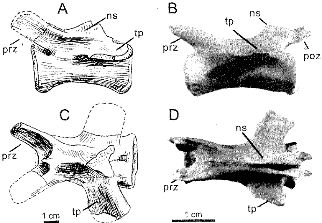
Fig. 21. Distal caudal vertebra of abelisauroids in lateral (A,B) and dorsal (C,D) views. A, C, indeterminate abelisauroid (K27/599), and B,D, Masiakasaurus knopfleri (from Carrano et al. 2002). Abbreviations: ns, neural spine; poz, postzygapophysis; prz, prezygapophysis; tp, transverse process.
